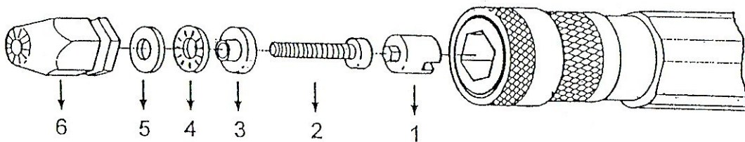
Complete nose piece assembly items 1 to 6
